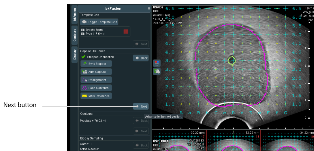
Figure 2-48. Realignment screen
