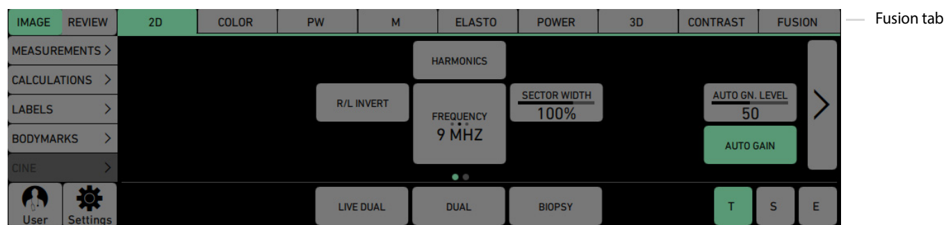
Figure 2-13. Fusion tab
