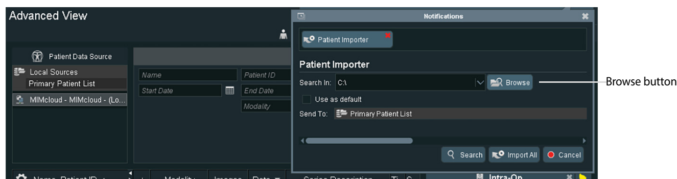
Figure 2-4. Browse button
