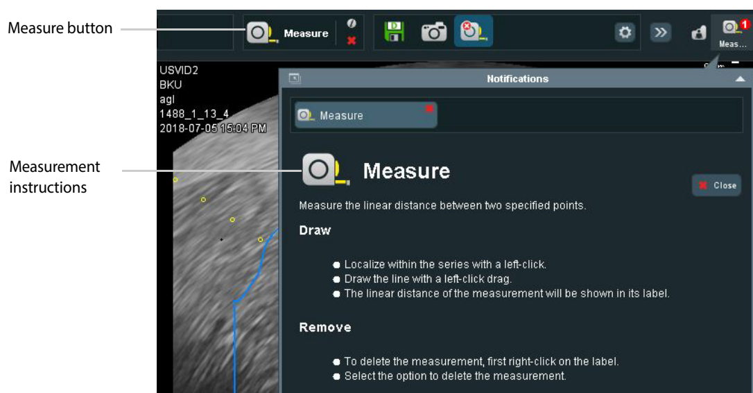
Figure 2-51. Measurement instructions
