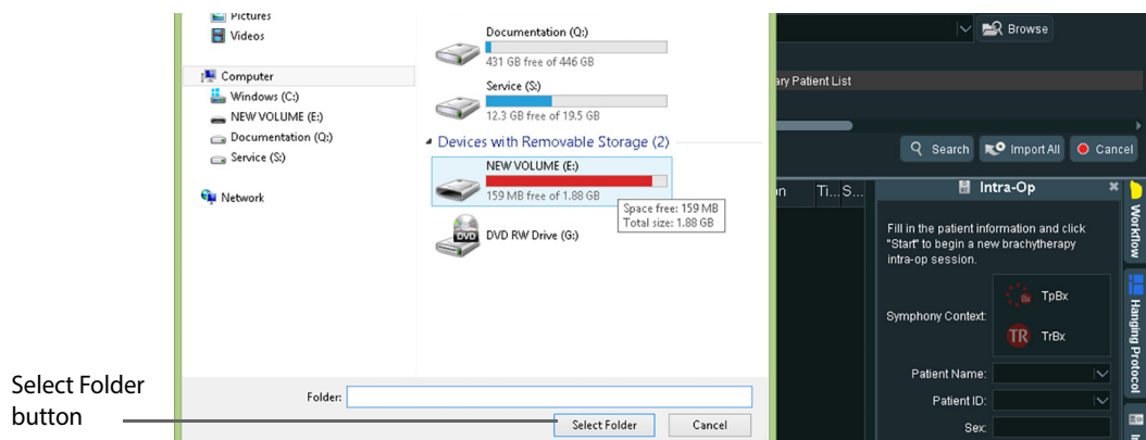
Figure 2-5. Browse screen
