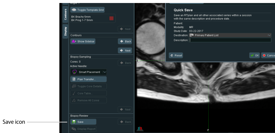
Figure 2-38. Save screen
