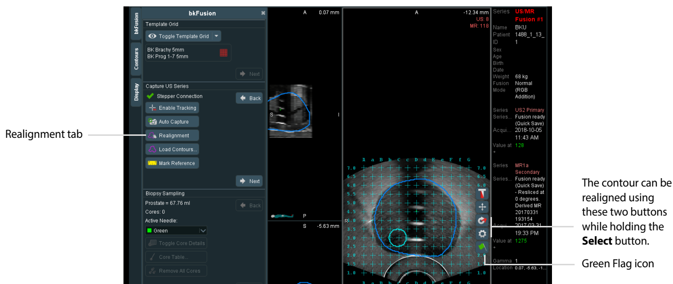
Figure 2-47. Realignment screen
