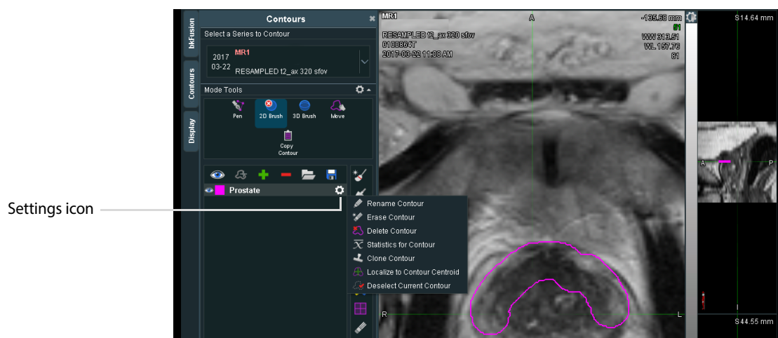
Figure 2-30. Contour settings
