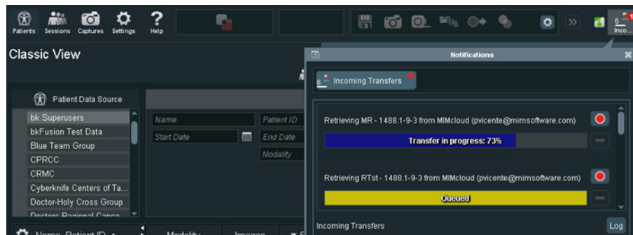
Figure 2-20. Data downloading
