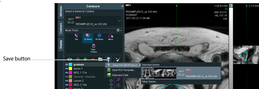
Figure 2-33. Save RTstructure
