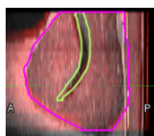
Figure 2-47. Realignment screen
