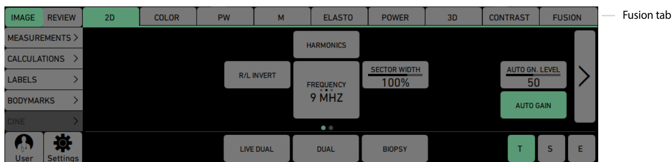
Figure 2-1. Fusion tab
