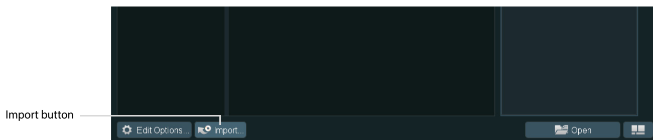
Figure 2-3. Import button
